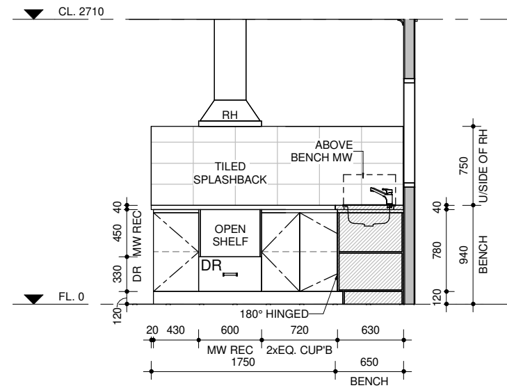
K1 KITCHEN A105 1 : 50
