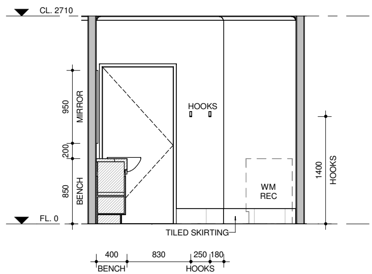
B4 B4 BATH A106 1 : 50
