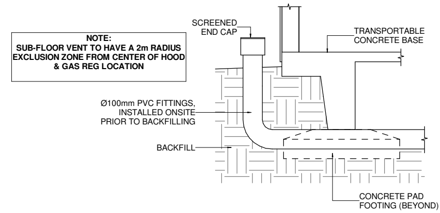
SV SUB FLOOR VENTILATION A107 1 : 20
