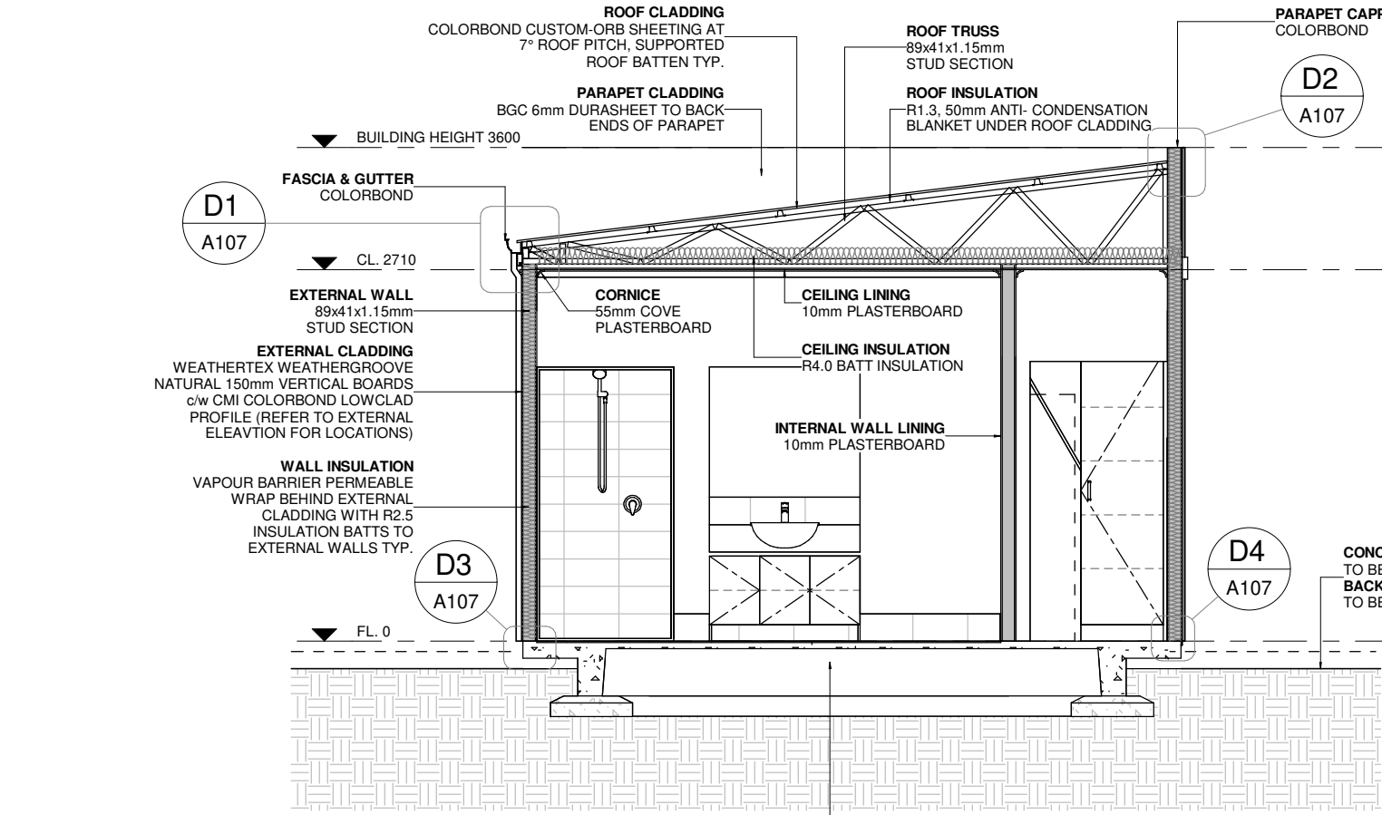
S1 BUILDING SECTION A107 1 : 50
