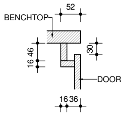
FG CUPBOARD FINGER GRIP DETAIL A105 1 : 10
