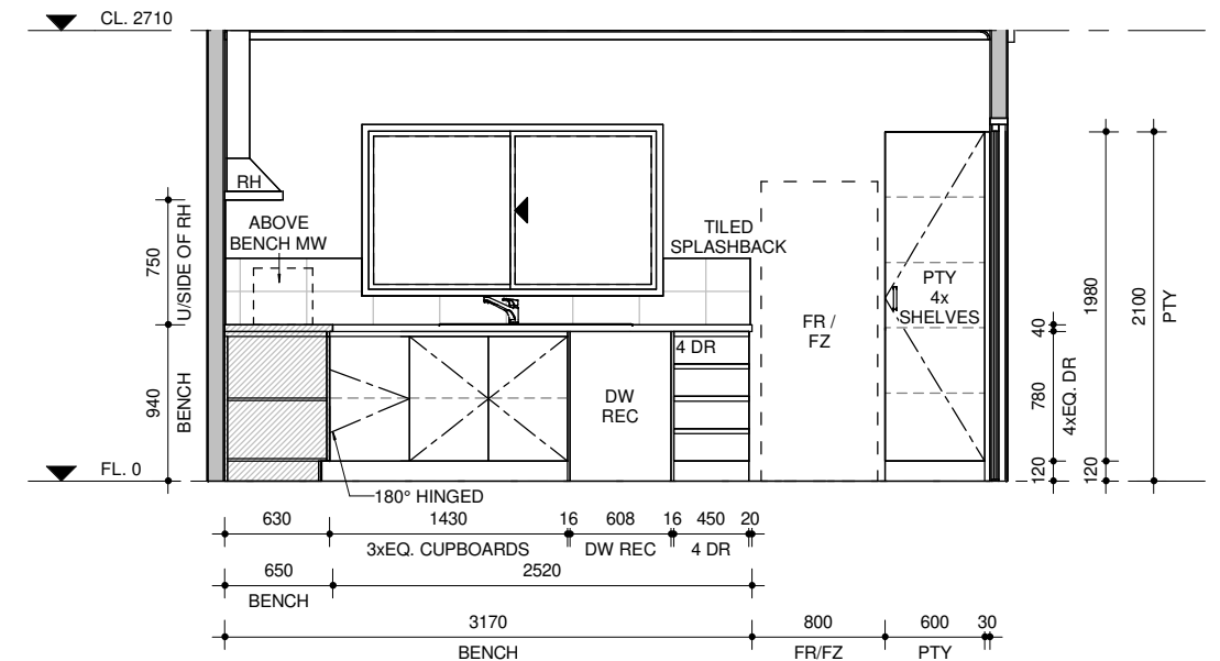
K2 KITCHEN A105 1 : 50
