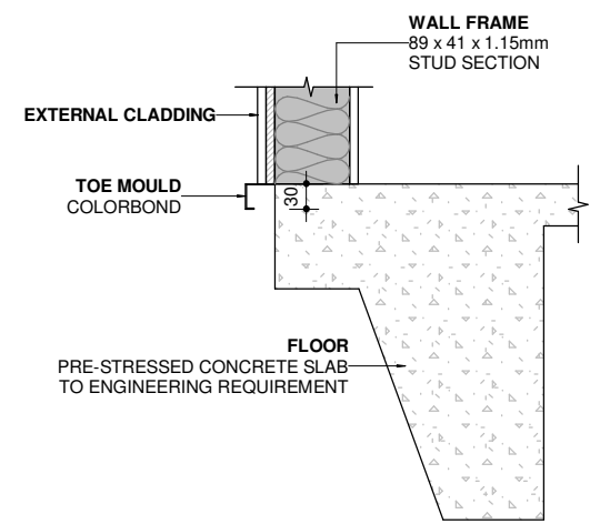
D3 TOE MOULD DETAIL A107 1 : 10
