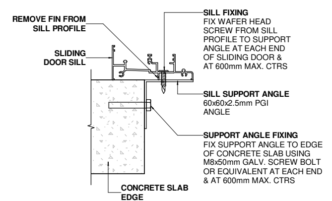
D4 SLIDING DOOR SILL SUPPORT DETAIL A107 1 : 5
